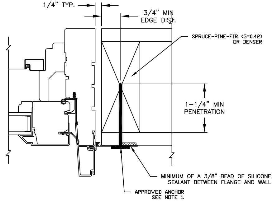
TYPICAL FLANGED WINDOW SIDE JAMB
