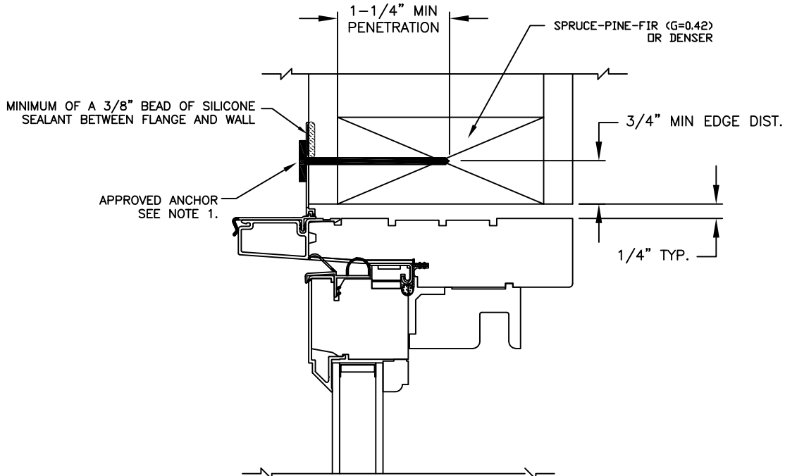
TYPICAL FLANGED WINDOW HEAD JAMB
